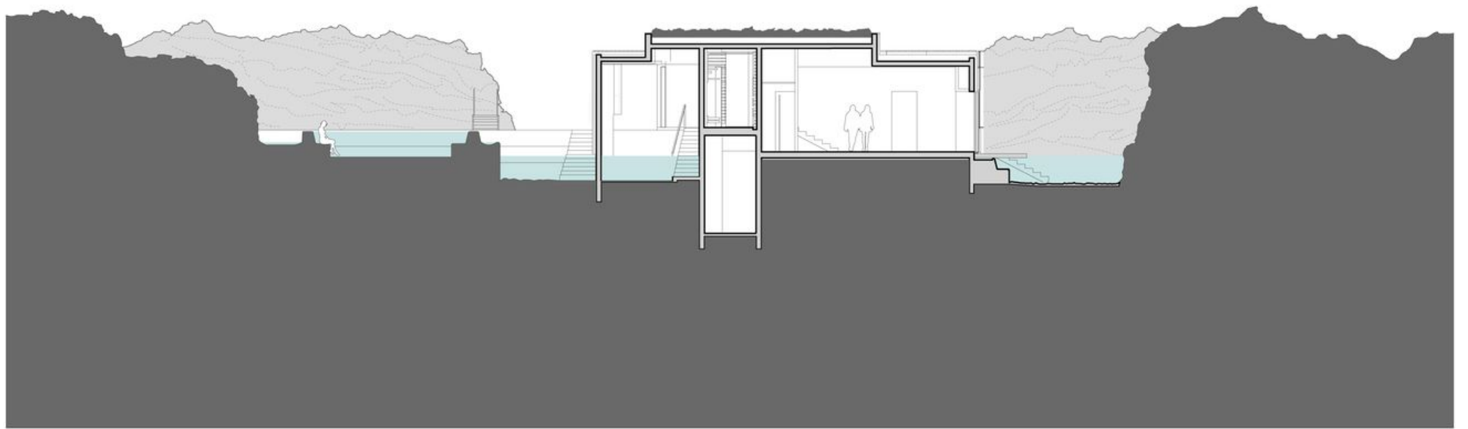
Section J-J
